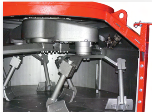
A80R head installed in access cover of planetary mixer
